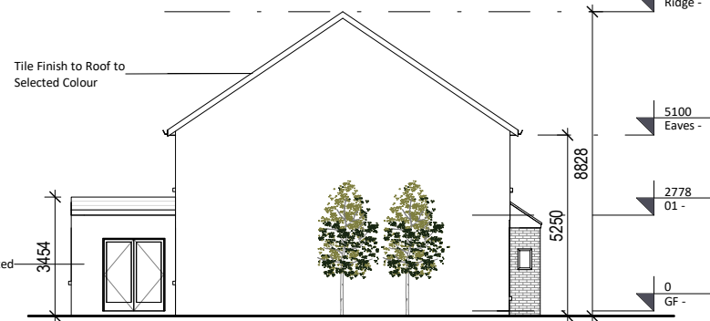
5 Gable Elevation Option A & B with Extension 1 : 200
