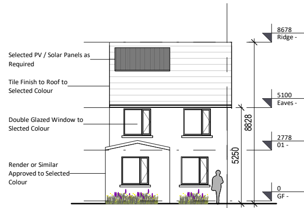
3 Rear Elevation Option A & B with Extension 1 : 200
