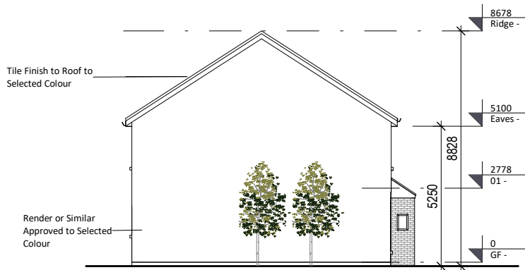
2 Gable Elevation Option A, B & C 1 : 200
